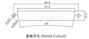
面板开孔 (Panel Cutout)
